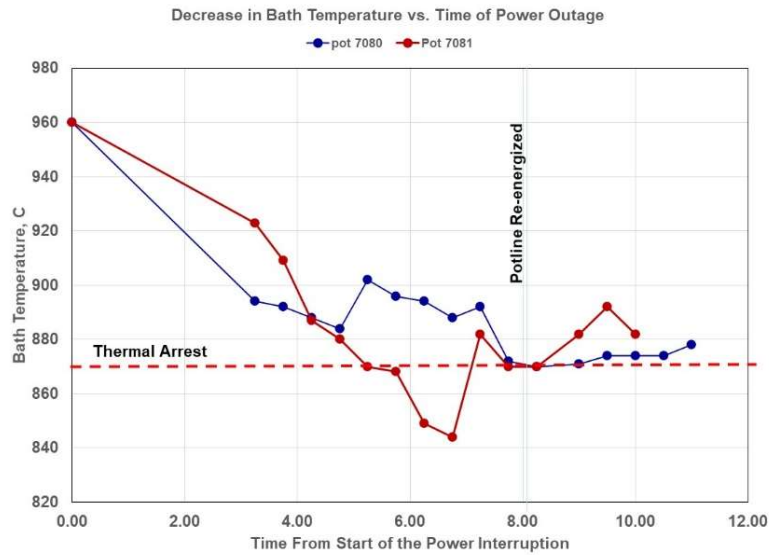
Figure 2. Bath cooling temperatures with a 3-hour thermal arrest at 870 °C during an 8.5-hour power interruption.
